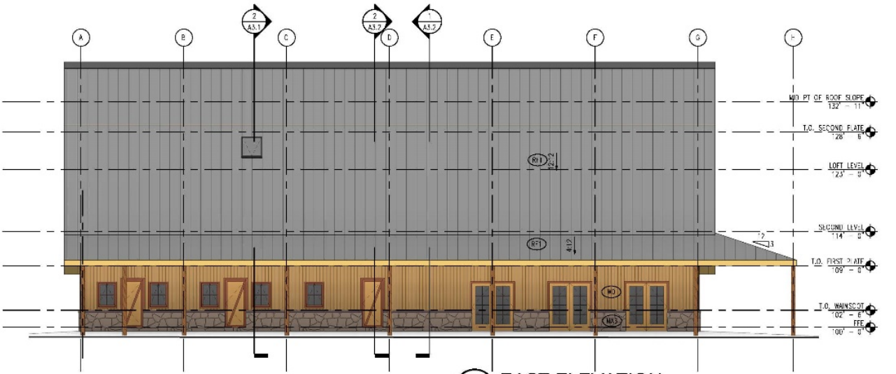
2 EAST ELEVATION A2.3 SCALE 1/8" = 1'-0"
