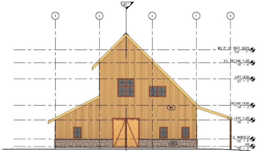
3 SOUTH ELEVATION A2.3 SCALE 1/8" = 1'-0"
