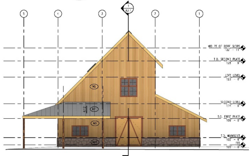
4 NORTH ELEVATION A2.3 SCALE 1/8" = 1'-0"
